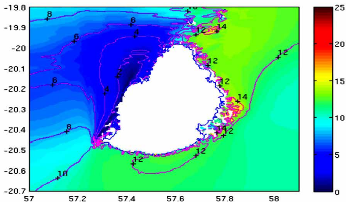
Figure 8-1: Wave density around Mauritius [Source: MRC]
