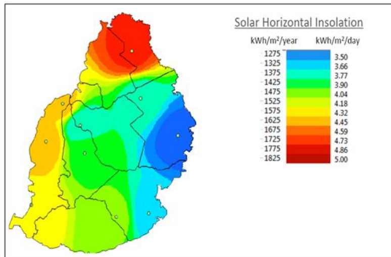
Figure 2-1: Solar potential by region [Source: R. Shea, 2017]
