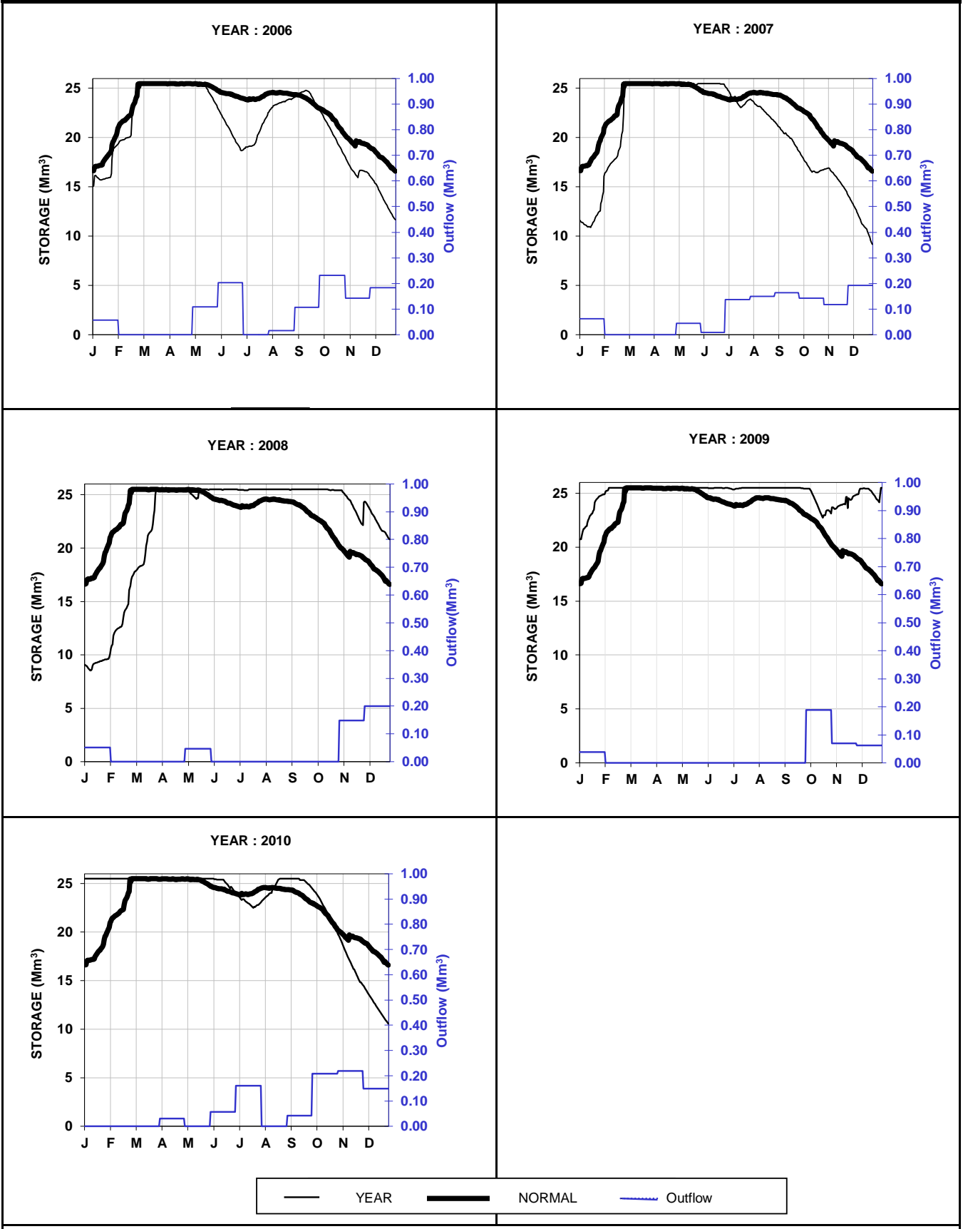
Fig. 5.5 Daily and Normal Storage Variation for Midlands
