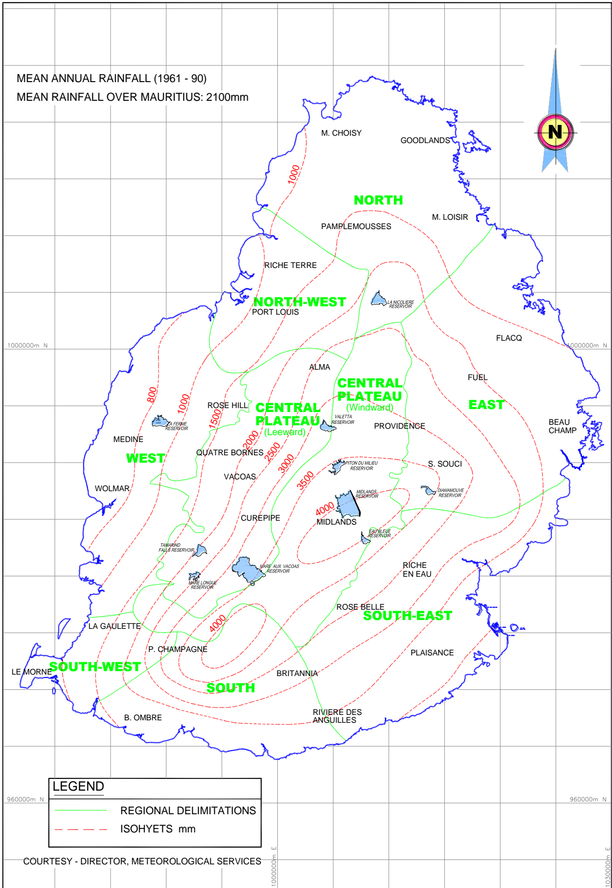
Fig. 2.3 Isohyetal Map of Mauritius (1961-1990)
